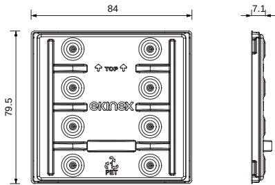
Dimensions [mm] - FF series
