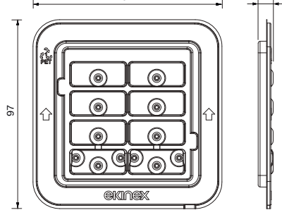
Dimensions [mm] - 20venti Surface series
