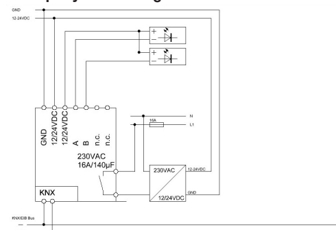
Exemplary circuit diagram AKD-0224V.02
