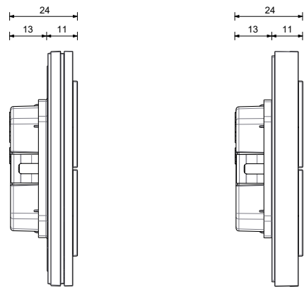
EK-ES2-TP Thermostat for no-frame mounting (NF series), completed with rocker and plate EK-PQS-...
